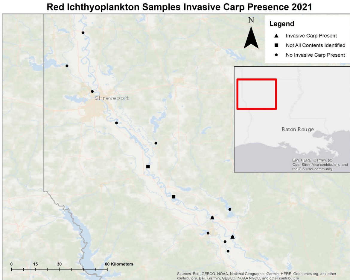
Figure 1. Sample locations where invasive carp have been identified (triangle), not all contents have been identified (squares), and where no invasive carp were identified (circles) as of January 2022.
