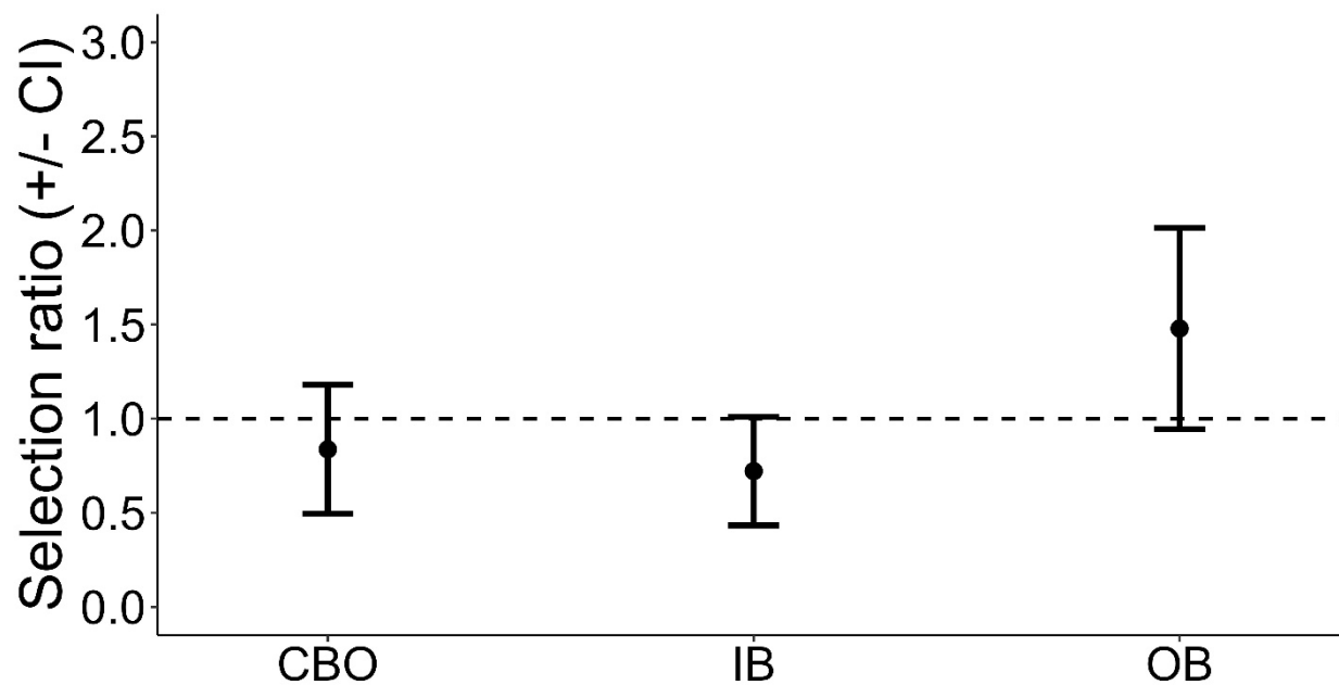
Figure 19. Selection ratios with 95% confidence intervals for macro-habitat [channel border open (CBO), inside bend (IB), and outside bend (OB)] in the Wabash and White rivers. Values greater than one indicate positive selection while values less than one indicate avoidance. These ratios were calculated using 305 detections of 108 unique individuals from 2021 to 2023.
