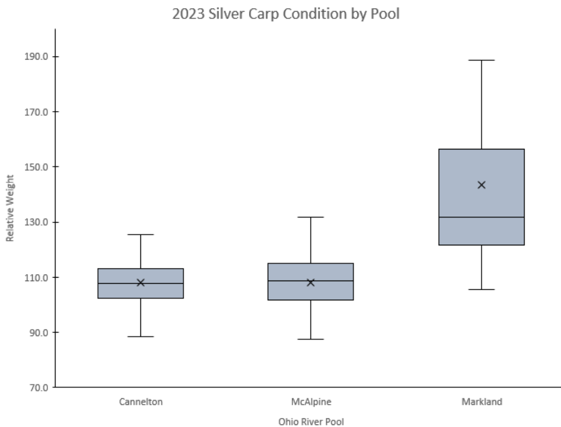
Figure 15. Relative weight ( W_r ) comparisons for Silver Carp collected in August – October 2023 from the Cannelton, McAlpine and Markland pools of the middle Ohio River. The standard weights needed for the W_r calculations were generated using the 50 th percentile regression methods outlined in Lamer et al, 2015.
